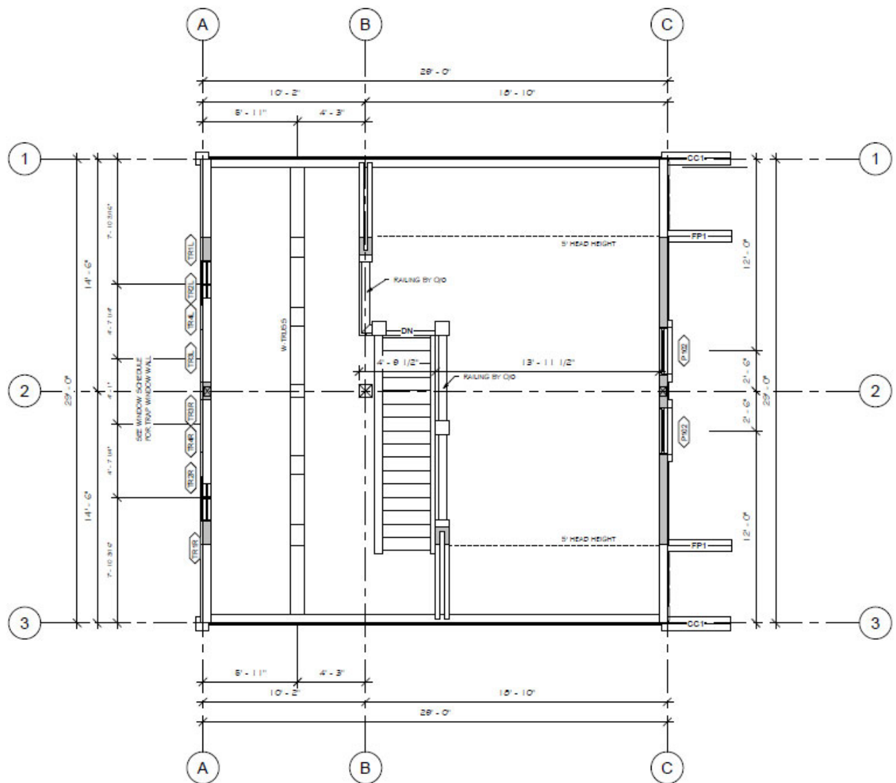
1 LOFT 1/4" = 1'-0"
